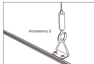
Accessory 1 is for pendant type of 6060/6161/6262 LED panel. Accessory 2 is for pendant type of 3012/3013/6012/6013 LED panel.
