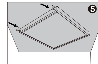
5. Fix the last frame with screw A.
